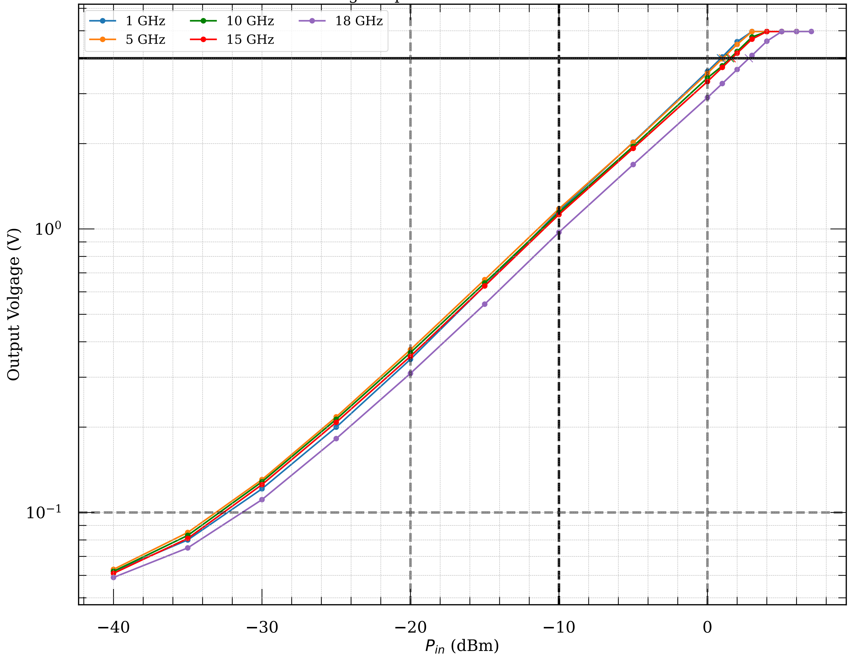
Measured voltage-to-power curve of detector module037v2
